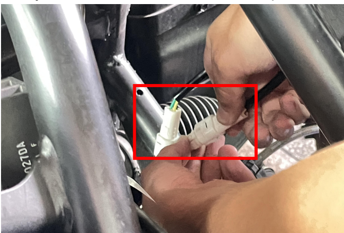
3. Reinstall the bracket of the installed lamp back into the original vehicle, connect the wiring harness plug of the headlight, and finally reinstall the hood. As shown in picture:
